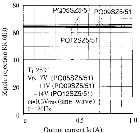
Fig.25 Ripple Rejection vs. Output Current
