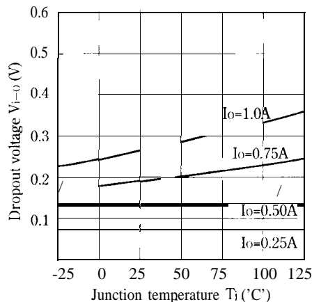
Fig.14-b Dropout Voltage vs. Junction Temperature (PQ05SZ1/11 Series)
